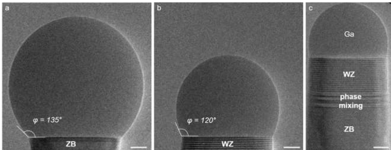
Figure 1. Impact of contact angle on the phase selection [10]. Images of a self-catalyzed GaAs NW recorded using the NanoMAX in situ TEM. The NW was grown by molecular beam epitaxy using the vapor-liquid-solid (VLS) method, where a liquid metal droplet (Ga in this case) catalyzes the growth of a solid NW from material provided from a gas phase. A large contact angle ( \varphi > 125^\circ ) results in the growth of ZB (a), while a small one corresponds to WZ (b). c Shows a NW having segments of the phases. Scale bars are 5 nm.
